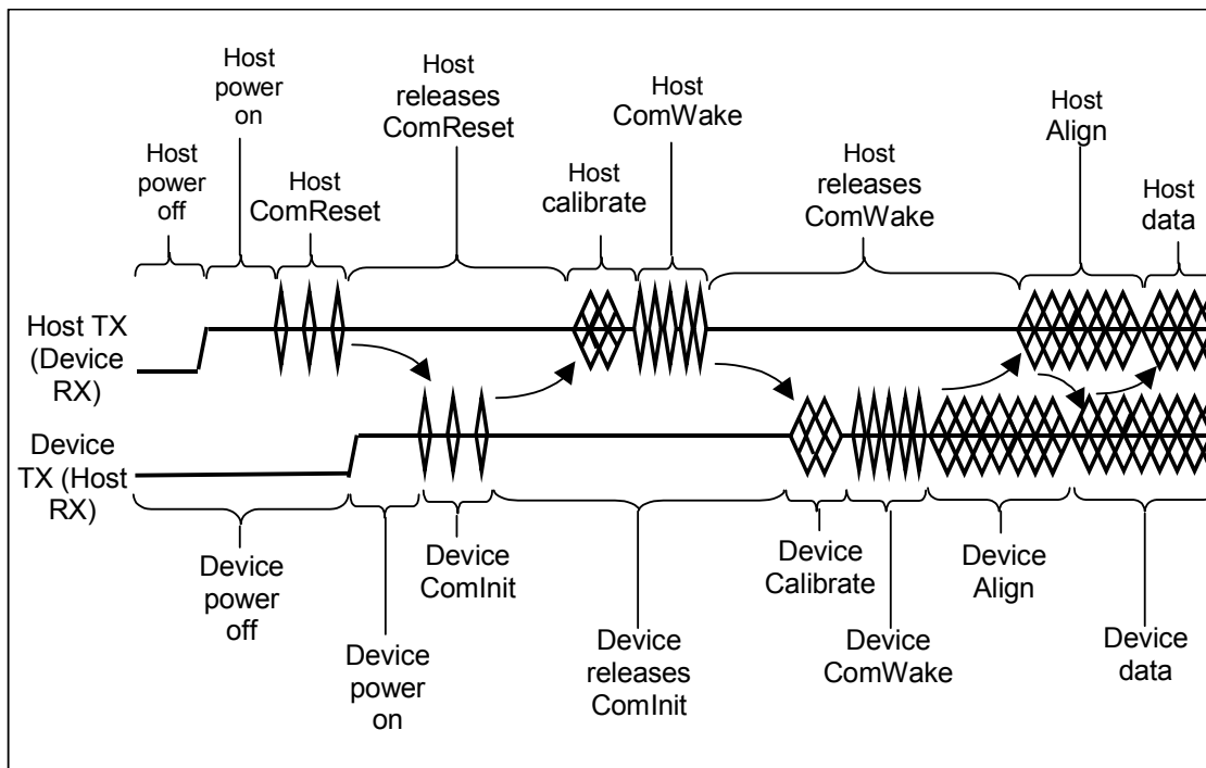
Figure 5.18 Power-on sequence
